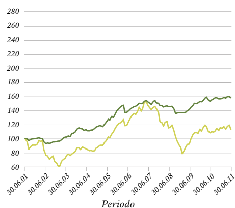
2001–2011 Performance in %
